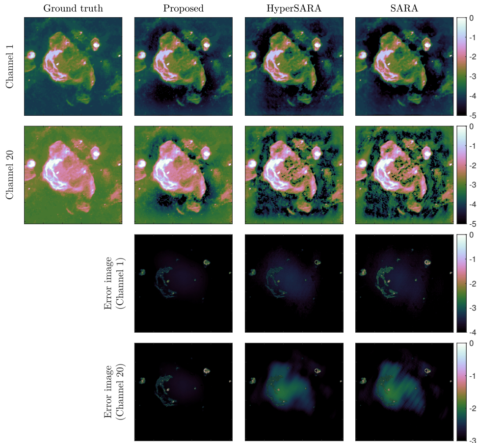
Fig. 1. Reconstructed (first two rows) and error images (last rows) displayed in log scale for the different approaches (in column: ground truth, proposed approach, HyperSARA and SARA). The reconstruction SNR for the displayed channels and per iteration computing time are: (proposed) [36.97/36.97 dB, 7.8 s], (HyperSARA) [SNR = 38.83/37.83 dB, 45 s], (SARA) [27.78/37.06 dB, 2.2 s]. Although the SNR reported for the proposed approach is smaller than the one of HyperSARA, the images obtained with the former approach show an overall improvement in the reconstruction quality of low intensity pixels for a much lower computing time than HyperSARA. The reconstruction performance of SARA is sub-optimal for wideband imaging since the correlation of the wideband data is not exploited, and given the nature of Fourier sampling in radio-astronomy where high Fourier modes are probed at higher frequency channels and low Fourier modes are probed at low frequency channels.
